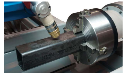
Rotary pipe/tube
